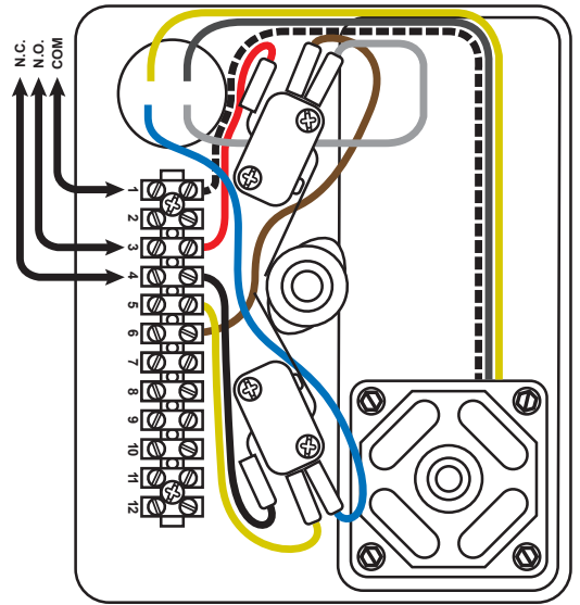
MBWA 1075 BLOWDOWN VALVE (TOP VIEW)
